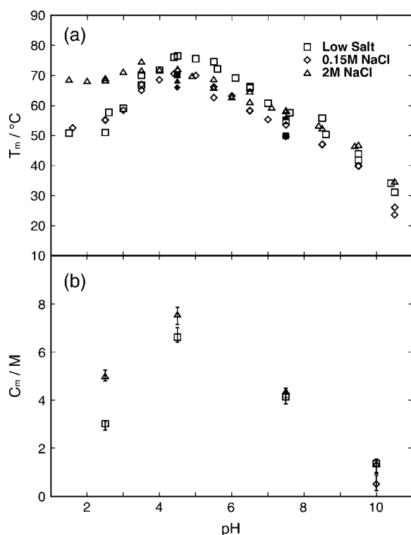
FIGURE 4 (a) Temperature at the denaturation midpoint, T_m , as a function of pH for the three different NaCl concentrations. Symbol key: \square , low salt; \diamond , 0.15 M NaCl; and \triangle , 2 M NaCl. Open symbols are for CD data and solid symbols are for DSC data. (b) Urea concentration at the denaturation midpoint, C_m , as a function of pH for the three different NaCl concentrations. Symbol key: \square , low salt; \diamond , 0.15 M NaCl; and \triangle , 2 M NaCl.
