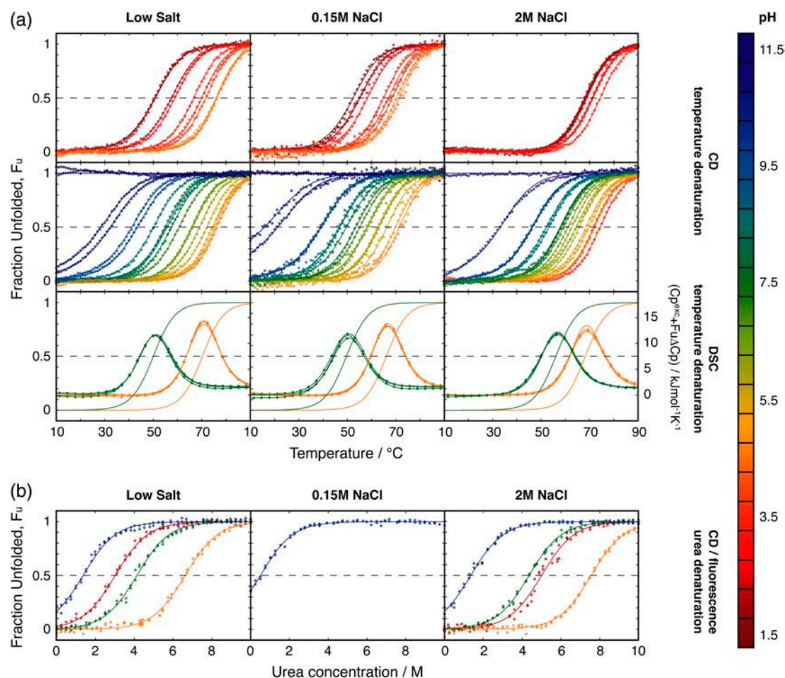
FIGURE 3 The pH-dependent stability. Experimental data points ( \diamond ) and fitted models (solid lines) are color-coded according to pH as indicated by the scale to the right. For the DSC data the fraction unfolded, F_U , is also displayed as a solid line. (a) Temperature denaturations of PGB1-QDD studied with CD (top two rows) and DSC (third row) at different pH values and three NaCl concentrations: (left) low salt; (middle) 0.15 M; and (right) 2 M. The top row shows temperature-denaturation curves at low pH values up to the pH with maximum stability at the respective salt concentration. The middle row shows data at high pH values down to the pH with maximum stability. (b) Urea denaturations studied with CD and fluorescence at different pH and the same three NaCl concentrations.
