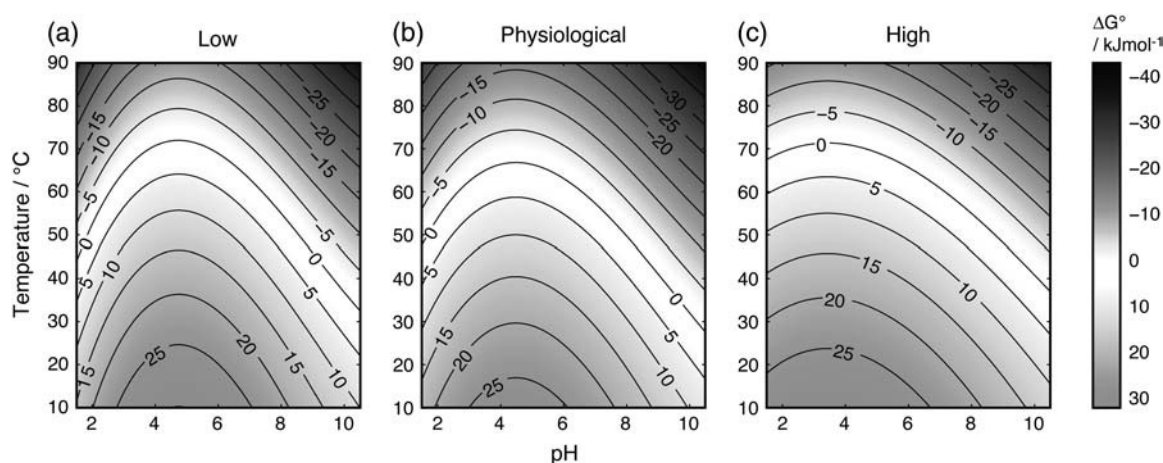
FIGURE 7 \Delta G^\circ contour maps calculated using fitted parameters from temperature denaturations at (a) low, (b) physiological, and (c) high salt concentrations.
